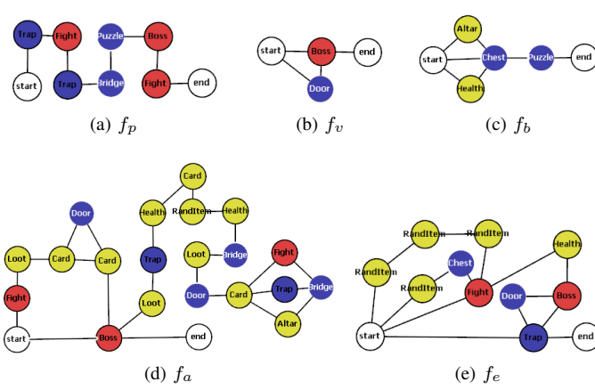
Fig. 3. Mission graphs of the fittest individuals evolved on single objectives.
