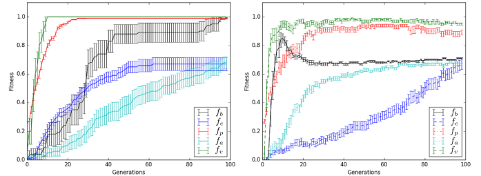
(a) Single objective evolution for each (b) Evolution towards a linear combination of the objective functions.
