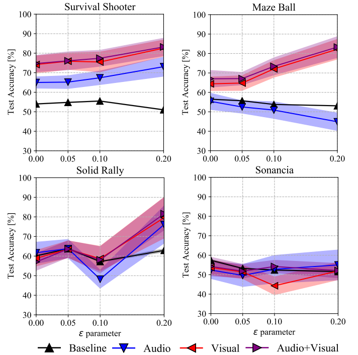
Fig. 5: Average classification accuracy (%) on the test set across the two modalities and different uncertainty threshold values ( \epsilon ). The time window is 0.5 seconds and shaded areas indicate the 95% confidence interval.
