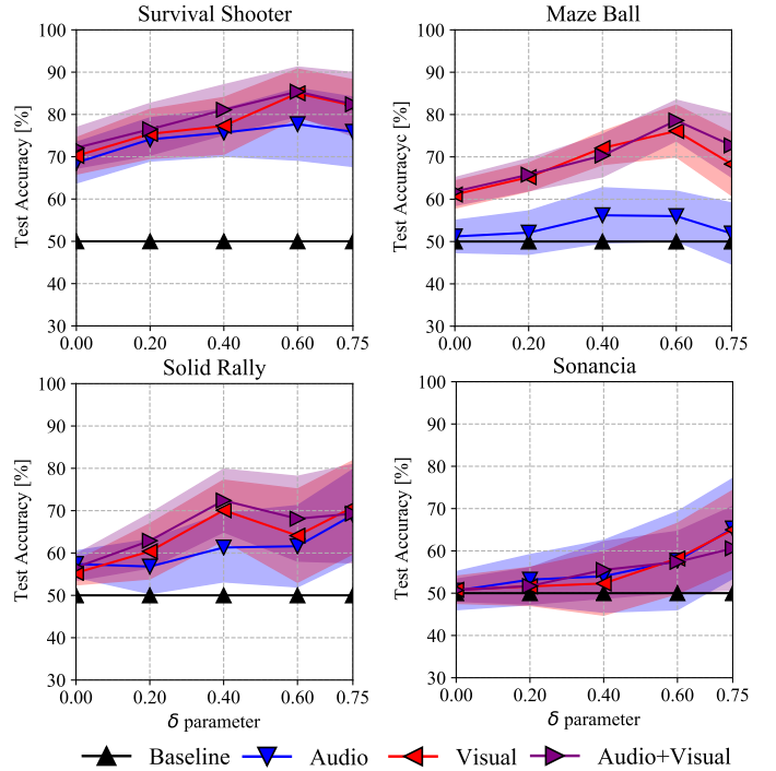
Fig. 6: Average accuracy (%) of the preference learner on test set across the two modalities and different uncertainty threshold values ( \delta ). The time window is 2.0 seconds and shaded areas indicate the 95% confidence intervals.
