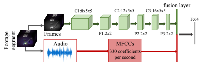
Fig. 3: The architecture of the proposed deep learning model. The convolutional, max pooling and fully connected layers are denoted by “C”, “P” and “F” respectively. The green stream corresponds to the processing of visual information, while the red stream to the audio information.
