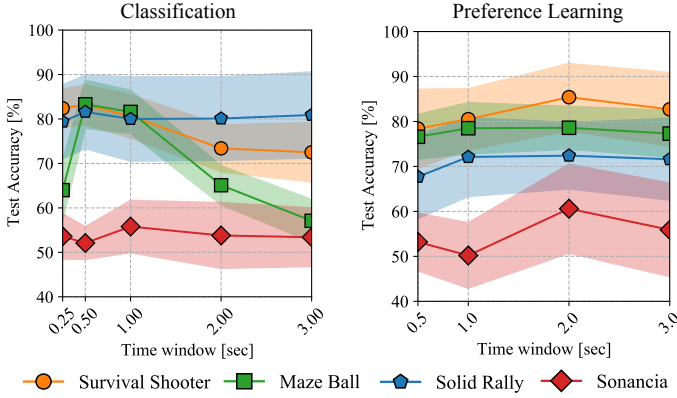
Fig. 7: Average accuracy (%) on test set for the best audiovisual model across different time windows, for classification and preference learning. Shaded areas indicate the 95% confidence intervals.
