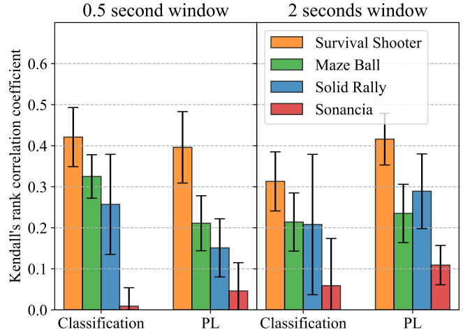
Fig. 8: Kendall's \tau across modelling approaches, games, and best time windows for each approach. Values are averaged from the leave-one-video out cross-validation and error bars denote the 95% confidence interval.
